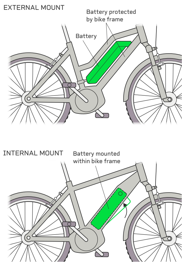
Figure 21: Recommended e-bike battery locations.
