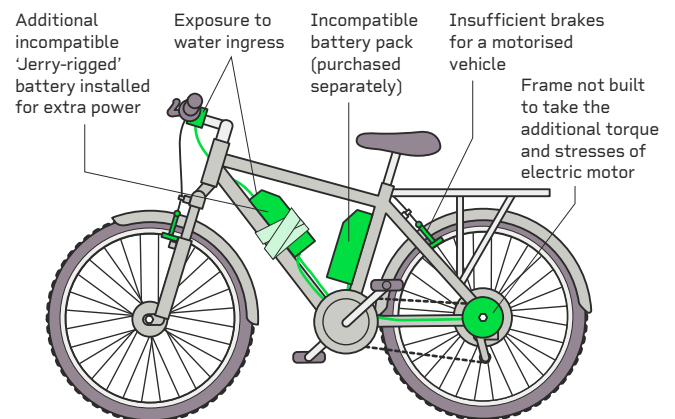
Figure 13: Associated risks of a DIY e-bike conversion.
