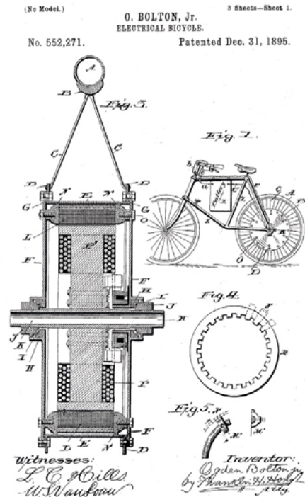
Figure 3: Extract from US Patent 552,271.
